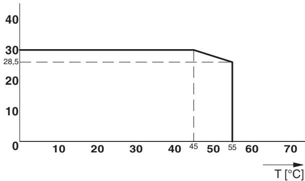
Figure 1 Derating diagram
