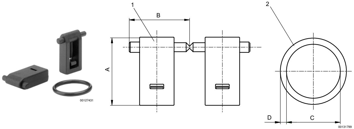
1) coupling clamp 2) O-ring
