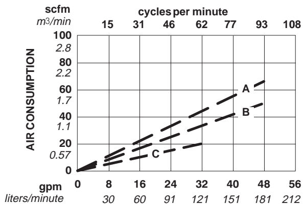
Air Consumption
