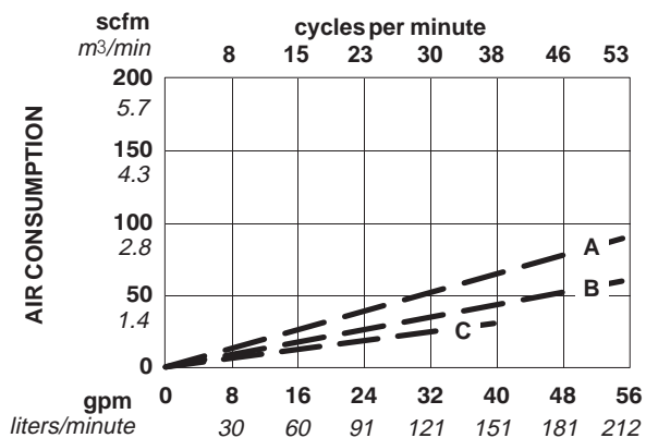
Air Consumption
