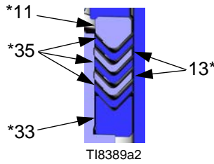
Piston Packings
