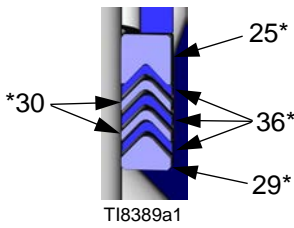
Throat Packings
