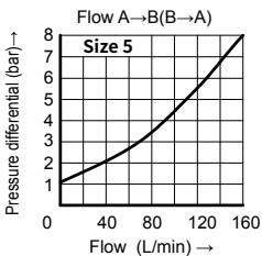
▲ Curve of rectifier plate type Z4S5
