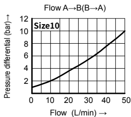
▲ Curve of rectifier plate type Z4S10
