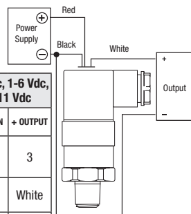
3 WIRE WIRING DIAGRAM EXAMPLE
