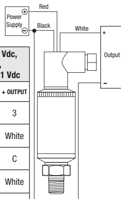
3 WIRE WIRING DIAGRAM EXAMPLE
