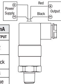
2 WIRE WIRING DIAGRAM EXAMPLE
