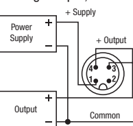
3 WIRE WIRING DIAGRAM EXAMPLE
