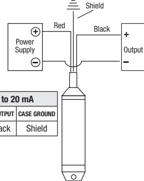
2 WIRE WIRING DIAGRAM EXAMPLE
