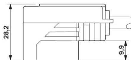
Valve connector, type B, side view
