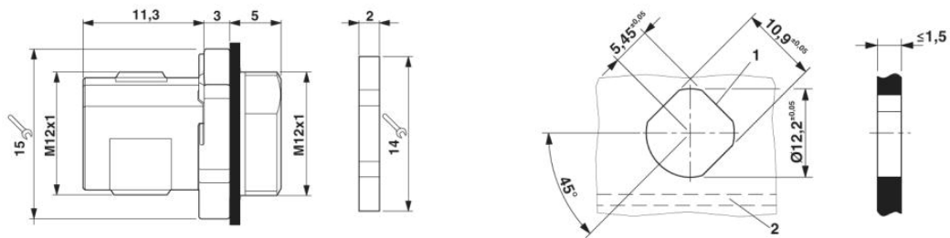
Housing cutout for M12 fastening thread, mounting panel with feed-through hole (alternative with surface as protection against rotation)
