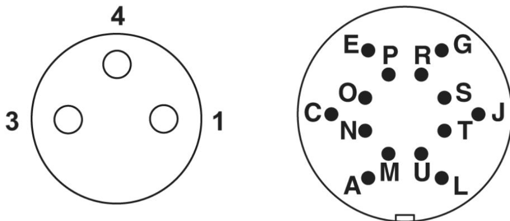
Connector pin assignment for M8 socket, 3-pos.
