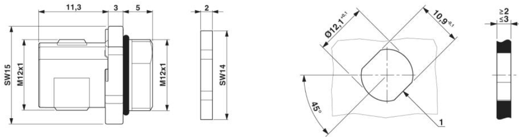
Housing cutout for M12 fastening thread, mounting panel with feed-through hole (alternative with surface as protection against rotation)
