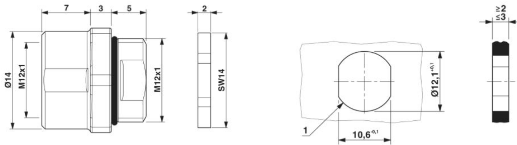
Housing cutout for M12 fastening thread, mounting panel with feed-through hole (alternative with surface as protection against rotation)
