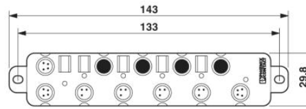
Top view (dimensions in mm)
