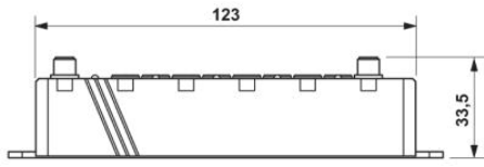
Side view (dimensions in mm)
