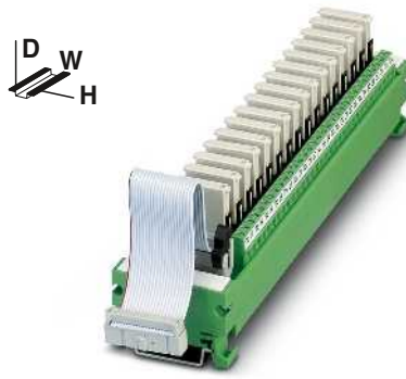
Output extension module with 16 miniature relays, 1 N/O contact
