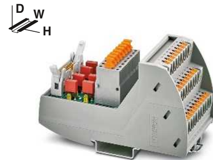
Interface module with fuses for 16-pos. mass termination block
