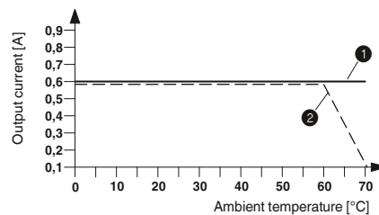
Derating curve for ELR H5-IES-SC-SWD/500AC-0.6 100% operating time
