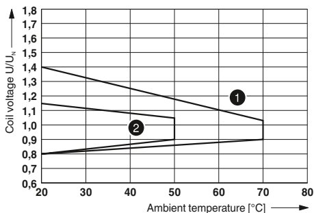
RIF-1 relay module with 2 PDT relay with manual operation
