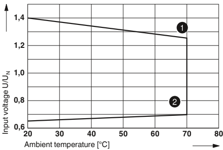
Permitted input voltage range for PLC-BSP-24DC/21RW (with REL-MR-18DC/21... relay)
