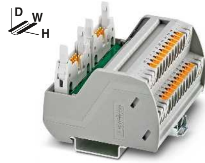
Passive interface modules for Allen Bradley ControlLogix with push-in connection
