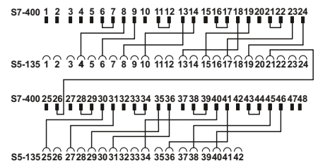
FLKM S135-460-4UA/I/S400 connection scheme
