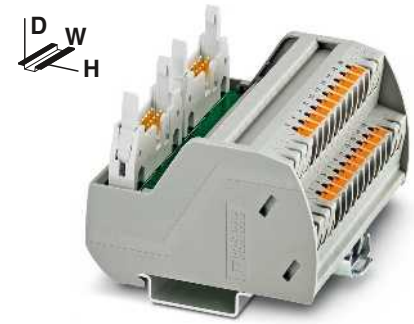
Passive interface modules for SIMATIC® S7-300 with push-in connection
