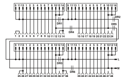
Connection scheme: FLKM 50/4-FLK14/PA-S400
