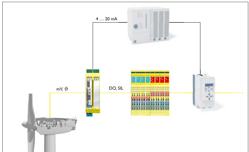
Application example: safety-related temperature monitoring in a wind power plant
