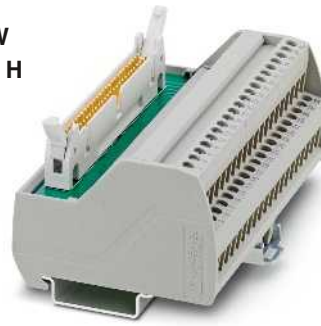
Passive interface modules for input/output, with specific marking and screw connection
