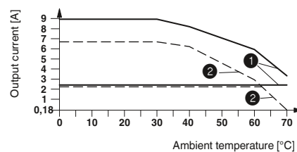
Derating curve for ELR H5-IES-SC-SWD/500AC-2 and ELR H5-IES-SC-SWD/500AC-9 100% operating time
