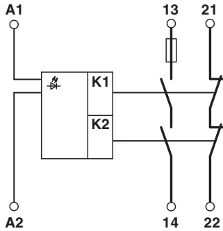
Figure 1 Block diagram
