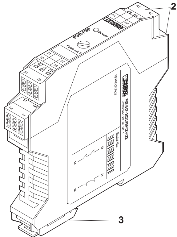
Figure 7 PSR-SPP- 24DC/FSP/1X1/1X2
