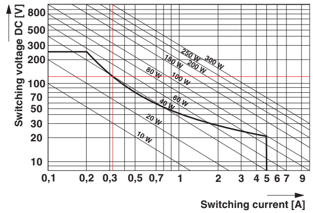
Figure 5 inductive load
